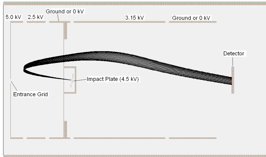
Figure 22. SIMION simulation of ions with 1 eV passing from a tilted impact plate to the detector in the reflectron mass spectrometer.
