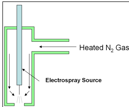
Figure 4. Desolvation with N_2 gas.
