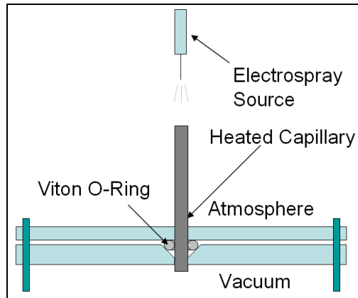
Figure 3. Heated desolvation capillary.
