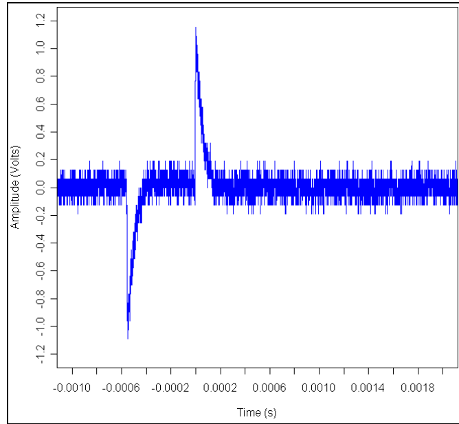
Figure 7. Image charge detector signal from a positively charged electrospay particle.
